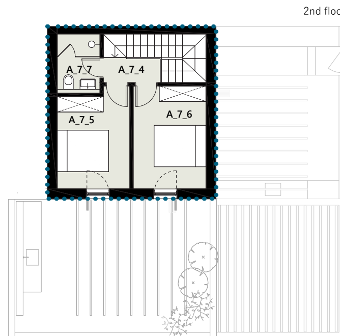
2nd floor
