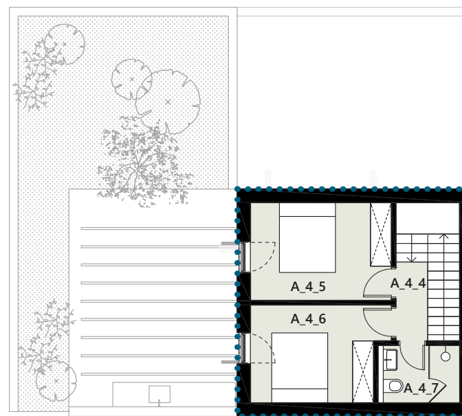
2nd floor
