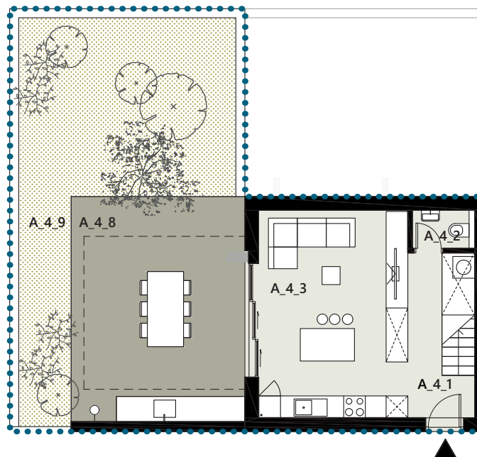
1st floor
